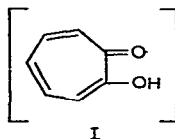
2-hydroxy-2,4,6-cycloheptatriene-1-one (I)
